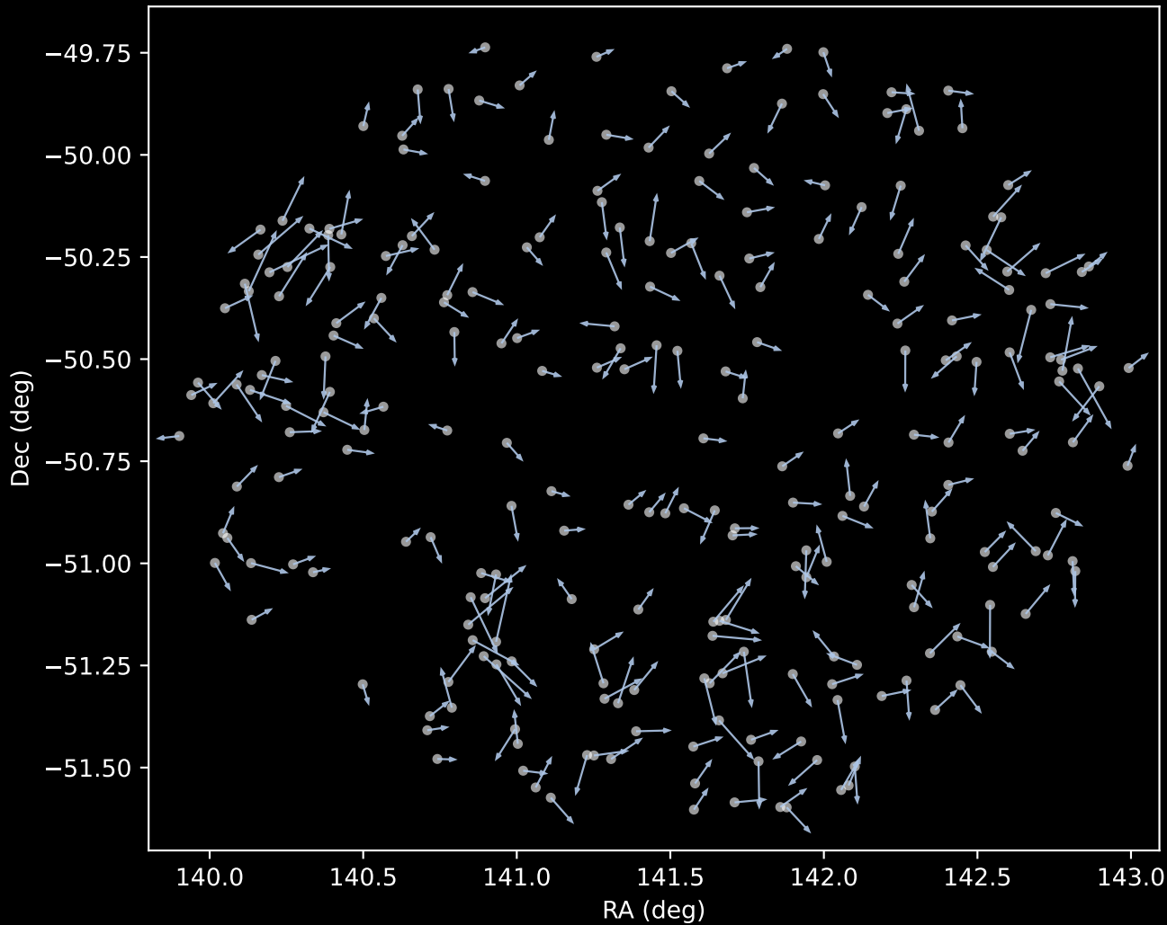
GALAH DR4 Cluster 1 Proper Motion Vectors (n=249)
