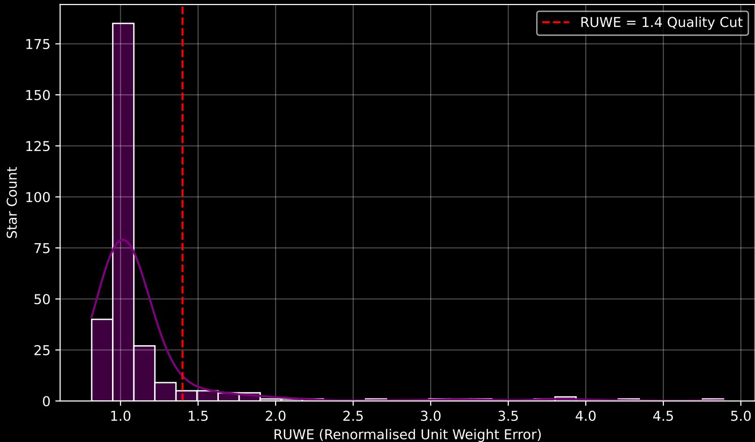
GALAH DR4 Field [6858] RUWE Distribution (n= 291)
