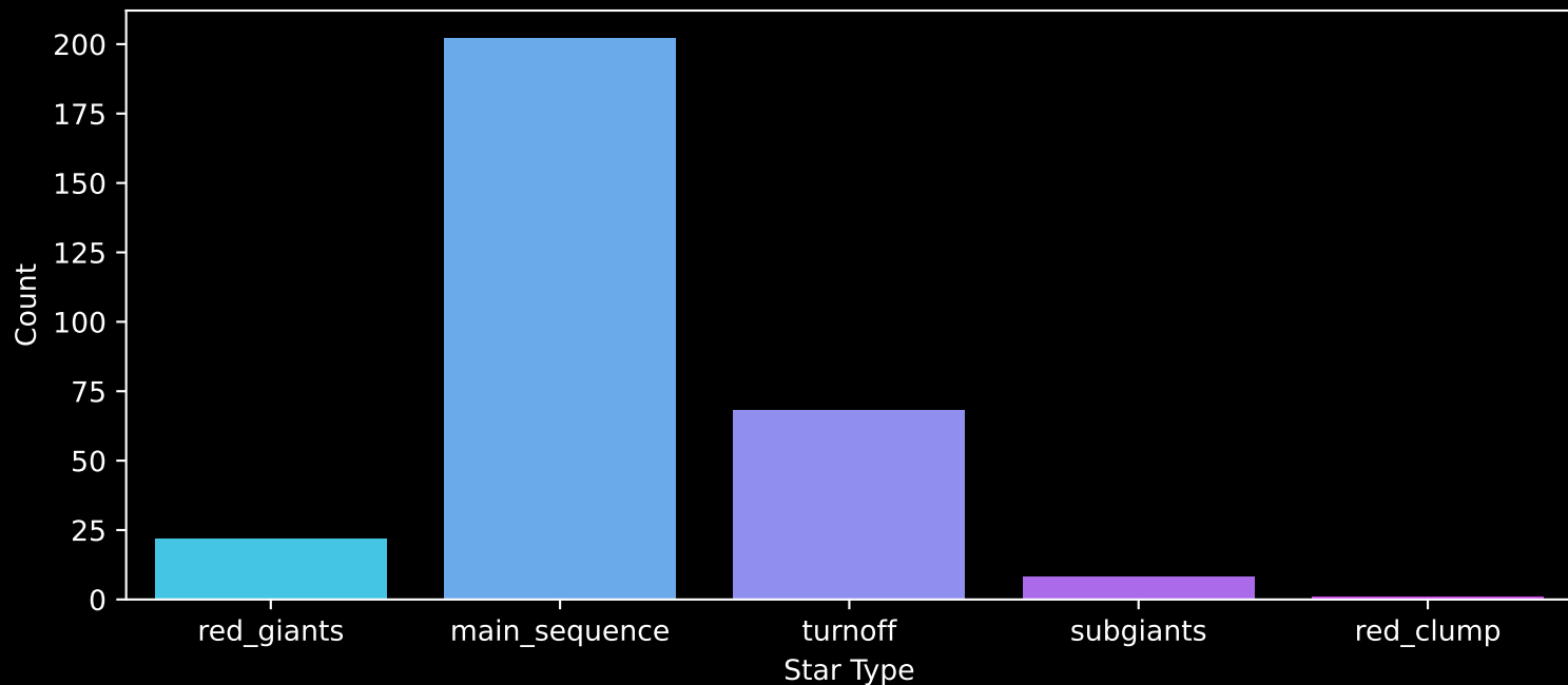
GALAH DR4 Field: [6858] Count plot of Star Type
